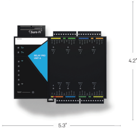
Relay Controller Interface Front
